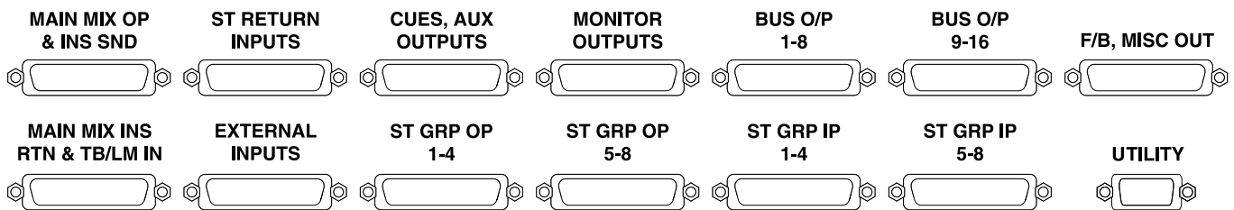
DB-25 Line Level Audio Connector Layout for the Master Section (all female connectors)
